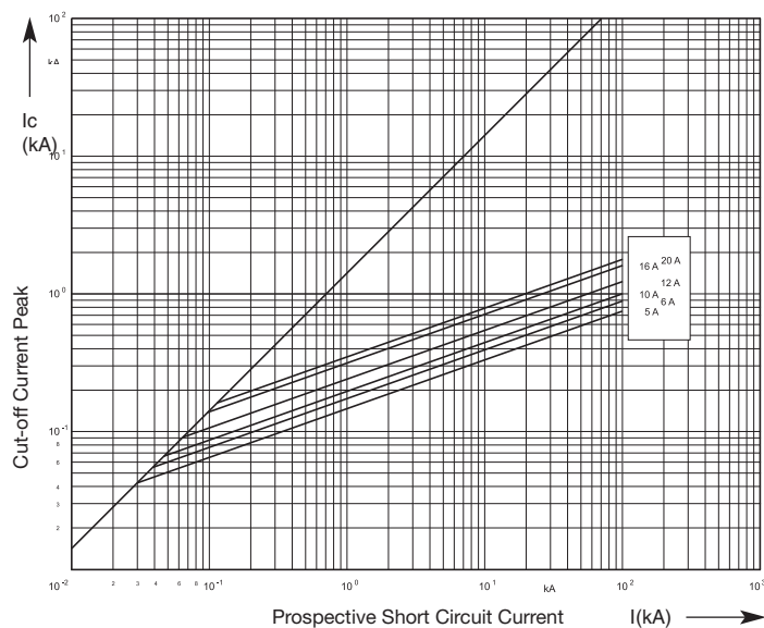
Cut-Off Characteristics
