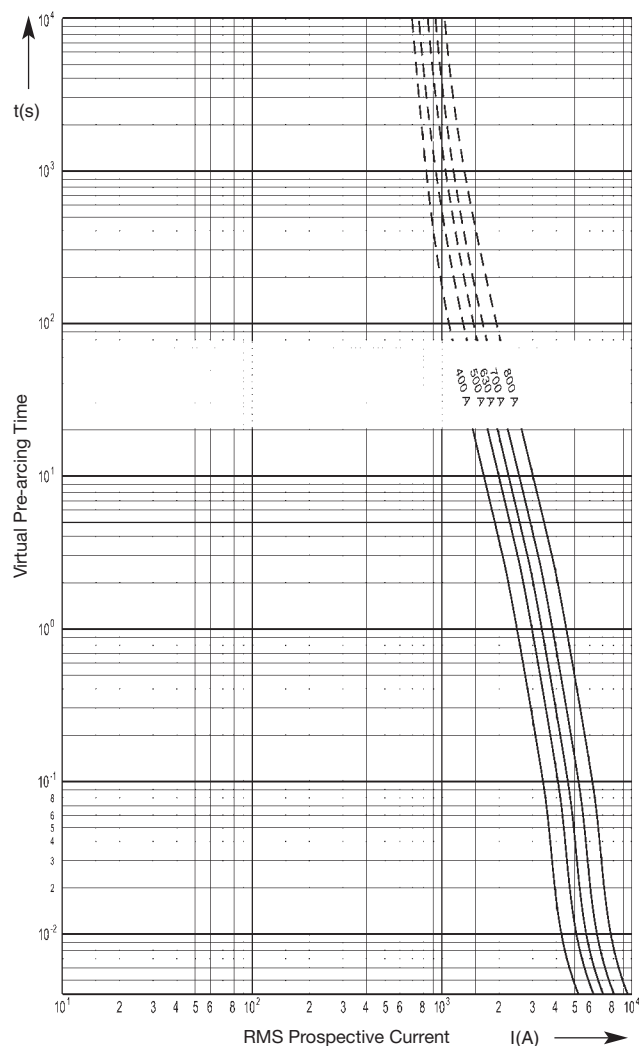
Time-Current Characteristics
